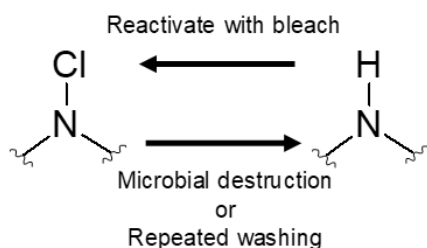
Figure 1: Use, inactivation, and reactivation of N-halamines.
