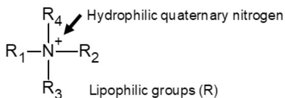
Figure 2: The base QAC structure produces surfactant properties.
