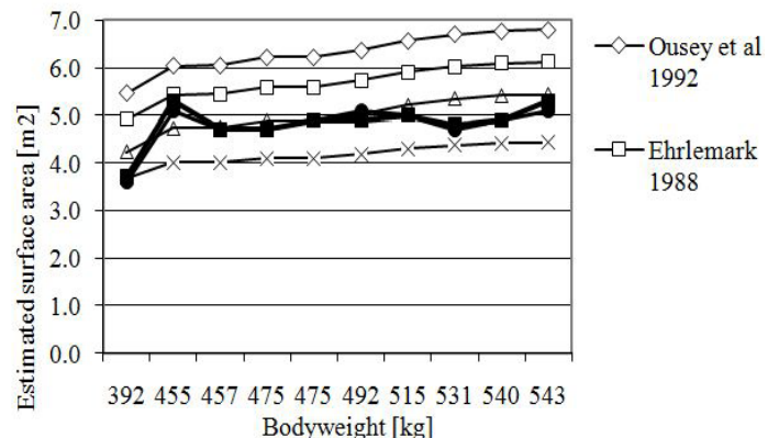
Figure 3: The diagram shows the estimated areas from the two equations No. 6: A 1 and No. 7: A 2 respectively) as compared to surface area as a function of body weight per different formulas found in literature. A=0.1m 0.67 , A=0.09m 0.67 , A=1.09+0.008mand A=0.13m 0.56 [4-7]. A is area in m 2 and m is body mass in kg.
